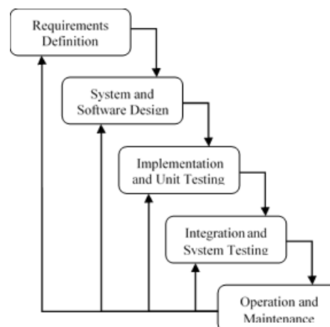
Gambar 2. Metode Waterfall
