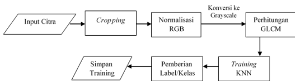
Gambar 3. Diagram alur training
