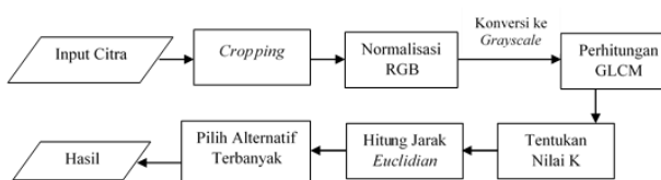
Gambar 4. Diagram alur testing
