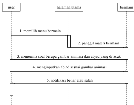
Gambar 4. Sequence Diagram Menu Bermain
