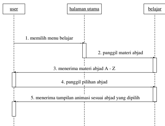
Gambar 3. Sequence Diagram Menu Belajar
