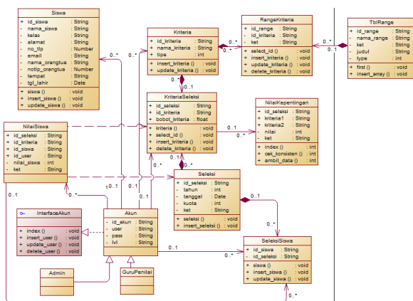
Gambar 3. Class Diagram
