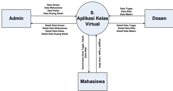
Gambar 3 DFD level 0
