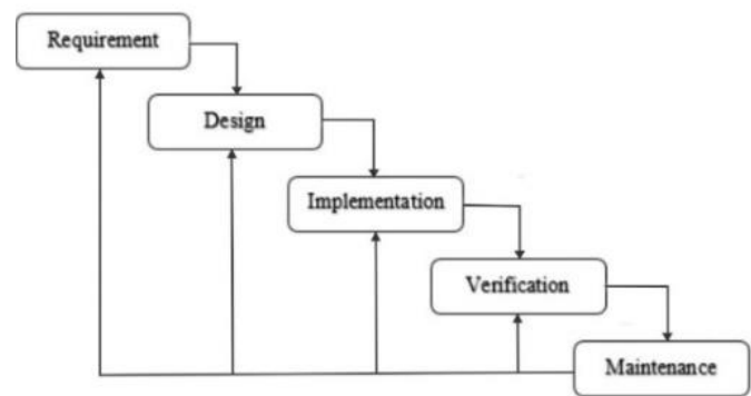
Gambar 6. Metode Waterfall
