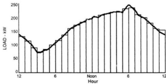
Gambar 2.1 Contoh Daily Load Curve
