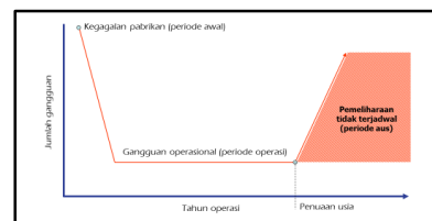
Gambar 4.6 Kurva Bathub
