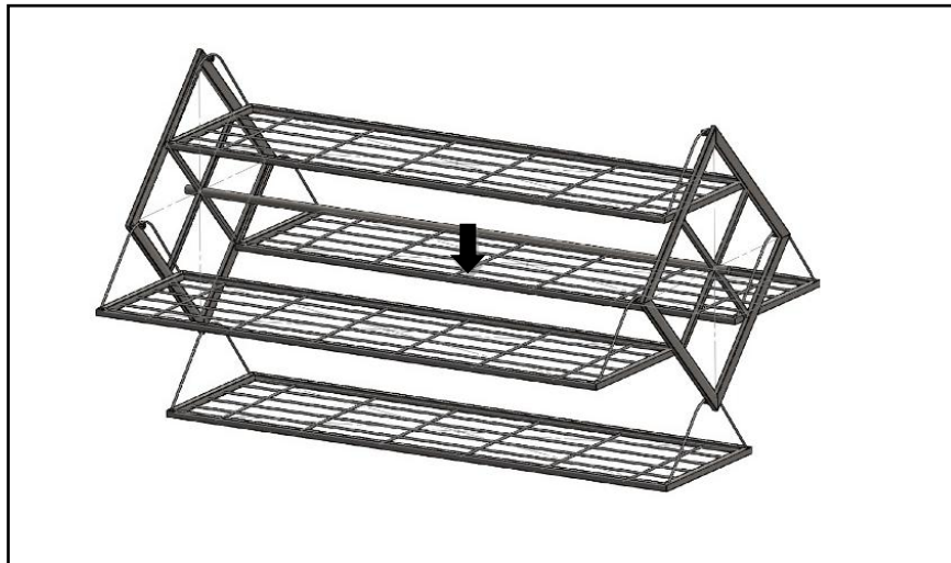
Gambar 5. Desain rak rotary mesin oven rotary
